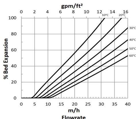
Figure 1: Backwash Expansion
