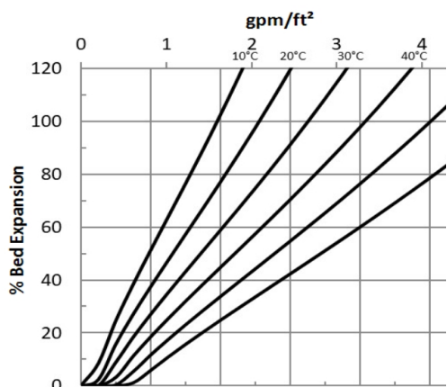
Figure 1: Backwash Expansion
