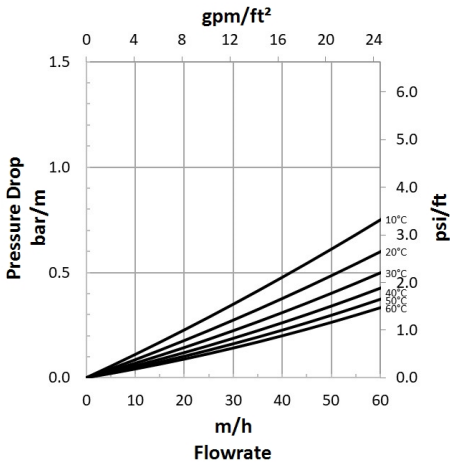
Figure 2: Pressure Drop Temperature = 10 – 60°C (50 – 140°F)
