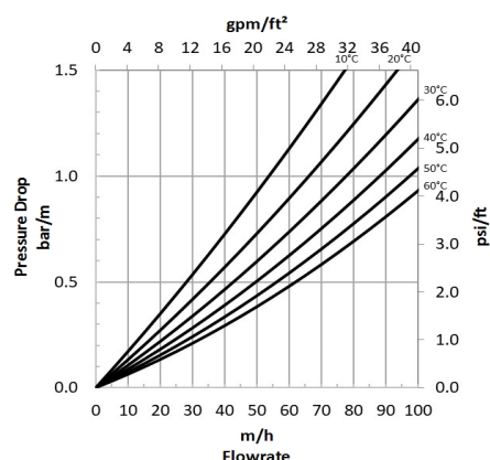
Figure 2: Pressure Drop
