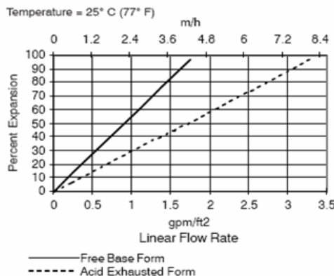
Figure 1: Backwash Expansion
