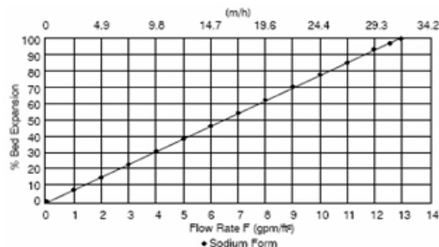
Figure 1: Backwash Expansion
